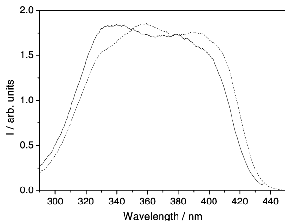
Fig. 5. Excitation spectra of alloxazinic ( \lambda_{em} = 430 nm, solid line) and isoalloxazinic ( \lambda_{em} = 540 nm, dashed line) forms of lumichrome in the presence of acetic acid ( c_{AA} = 0.09 mol dm ^{-3} ) in 1,2-dichloroethane.
