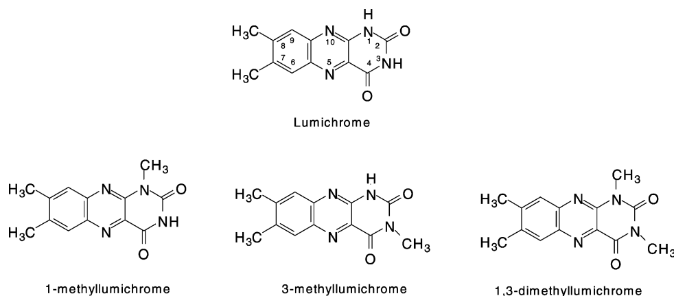
Fig. 1. Structure of the lumichrome, 1-methylalumichrome, 3-methylalumichrome and 1,3-dimethylalumichrome studied.
